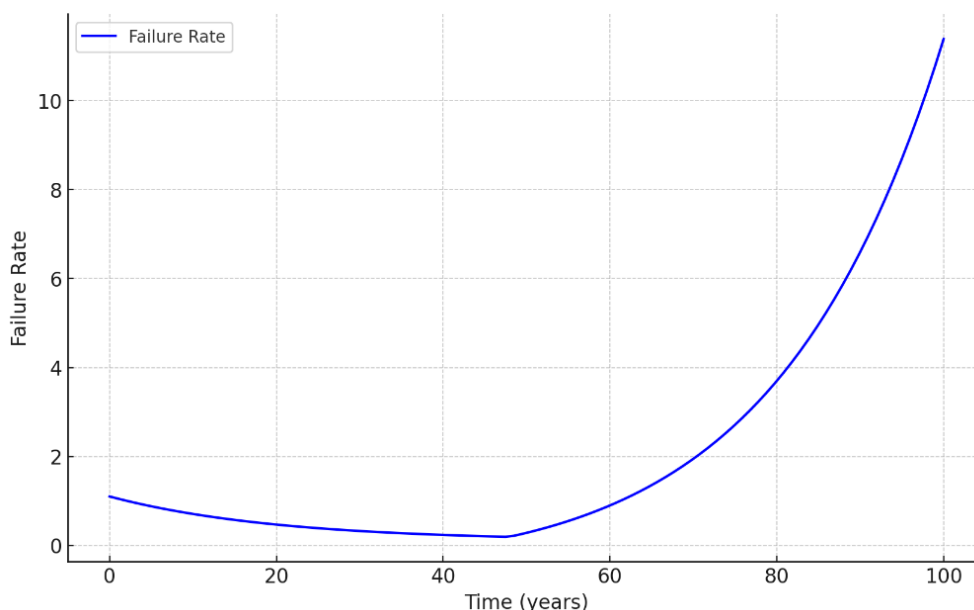
Fig. 1. Equipment Failure Rate Over Time (Bathtub Curve)
