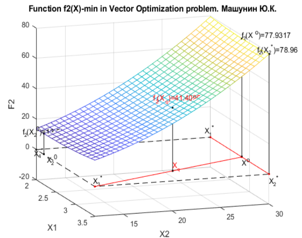
Figure 8. The second characteristics of the f_2(X) technological process in physical units in the three-dimensional coordinate system \{x_1, x_2 \text{ and } f_2(X)\}
