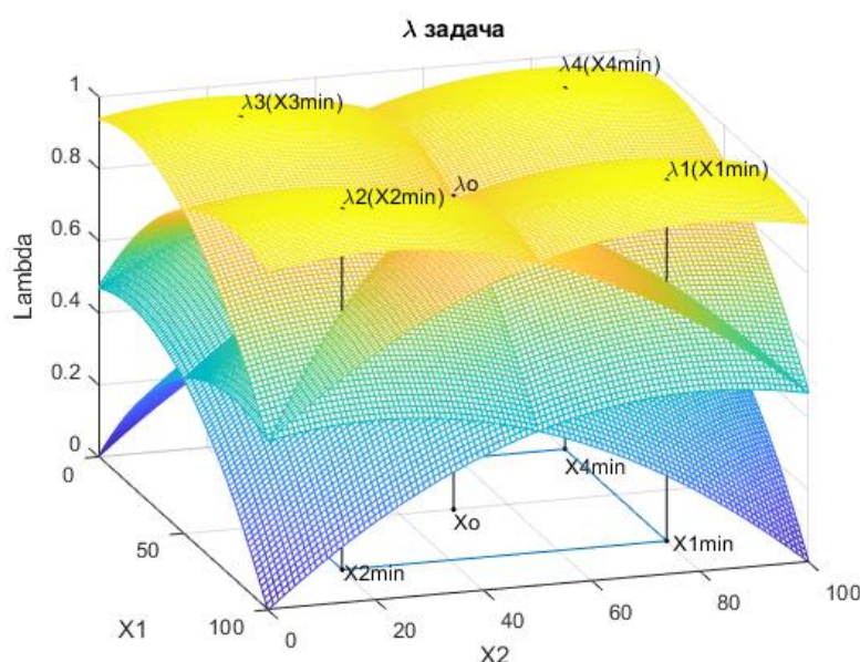
Figure 4. Results of the solution to VPLP (65)-(69) and (70): functions: \lambda_1(X), \lambda_2(X), \lambda_3(X) , and \lambda_4(X) , points of an optimum of X^o and \lambda^o
