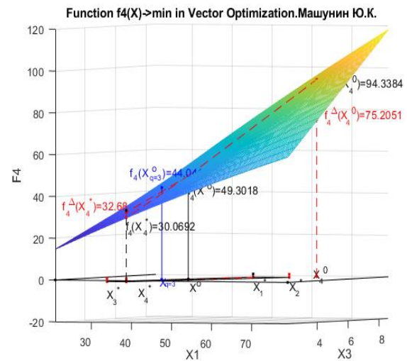
Figure 19.k3. Function f_4(X) with the priority of the third criterion in the two-dimensional coordinate system x_1 x_3 and a geometric interpretation of the function f_4(X_{3,q=3}) in the coordinate system x_1 x_2 x_3 x_4 .
