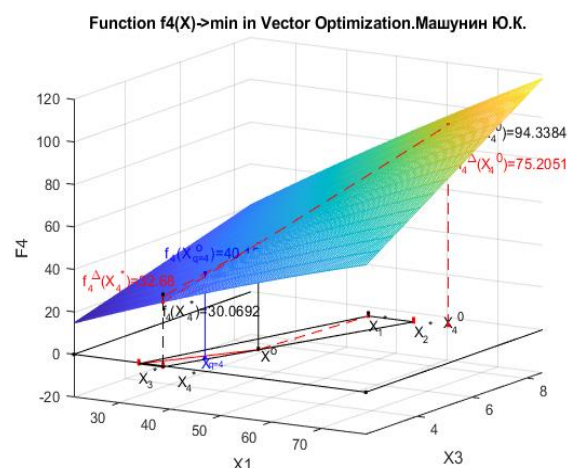
Figure 19.k4. Function f_4(X) with the priority of the fourth criterion in the two-dimensional coordinate system x_1 x_3 and a geometric interpretation of the function f_4(X_{4,q=4}) in the coordinate system x_1 x_2 x_3 x_4 .
