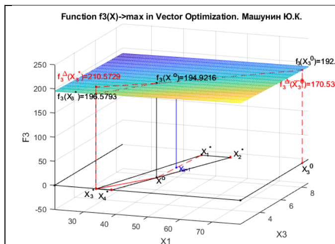
Figure 18.k1. Function f_3(X) with the priority of the first criterion in the two-dimensional coordinate system x_1 x_3 and a geometric interpretation of the function f_3(X_{1,q=1}) in the coordinate system x_1 x_2 x_3 x_4 .
