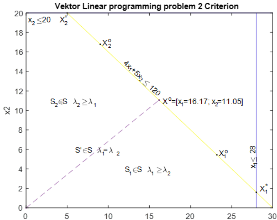
Figure 1. Solution of VPMP (57) and (58).
