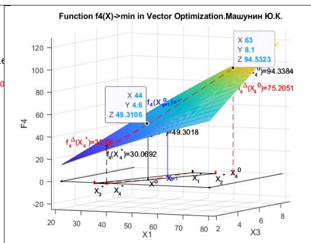
Figure 19.k1. Function f_4(X) with the priority of the first criterion in the two-dimensional coordinate system x_1 x_3 and a geometric interpretation of the function f_4(X) in the coordinate system x_1 x_2 x_3 x_4 .
