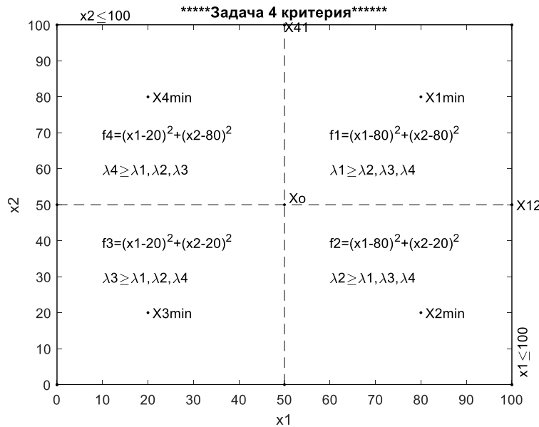
Figure 3. A geometrical interpretation of VPMP (55)-(59). The results of the solution to VPMP
