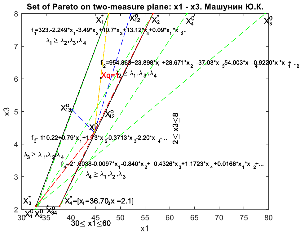
Figure 11. The permissible set of points S in the coordinates \{x_1, x_3\} . A set of Pareto-optimal points S^0 \subset S , bounded by the points X_1^*, X_2^*, X_3^*, X_4^* and the local S_1^0 between X_1^*, X_{13}^0, X^0, X_{12}^0, X_1^* in the two-dimensional coordinate system \{x_1, x_3\} .
