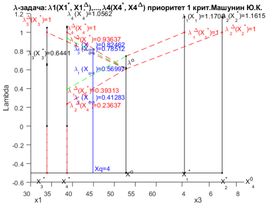
Figure 15.k4. \lambda -problem in the coordinate system x_1 x_3 and \lambda .
