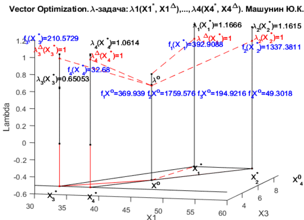
Figure 14. \lambda -problem in the coordinate system x_1 x_3 and \lambda . Geometric interpretation of the results of solving four criteria in relative and physical units.
