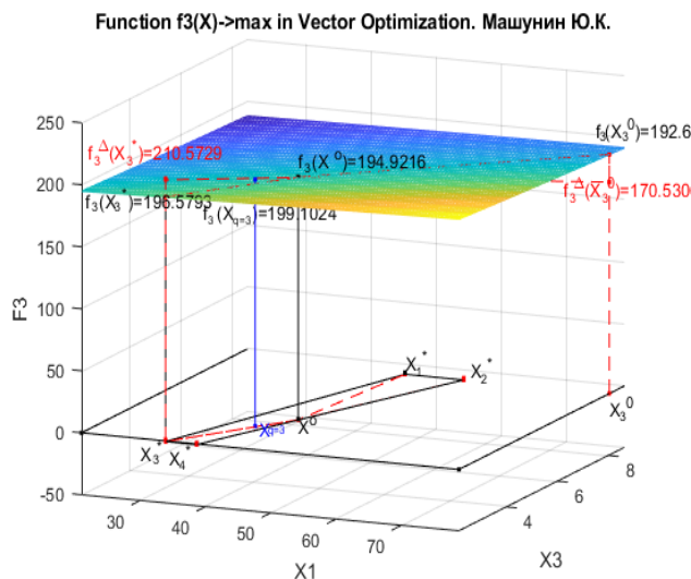
Figure 18.k3. Function f_3(X) with the priority of the third criterion in the two-dimensional coordinate system x_1 x_3 and a geometric interpretation of the function f_3(X_{3,q=3}) in the coordinate system x_1 x_2 x_3 x_4 .
