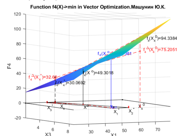
Figure 19.k2. Function f_4(X) with the priority of the second criterion in the two-dimensional coordinate system x_1 x_3 and a geometric interpretation of the function f_4(X_{2,q=2}) in the coordinate system x_1 x_2 x_3 x_4 .
