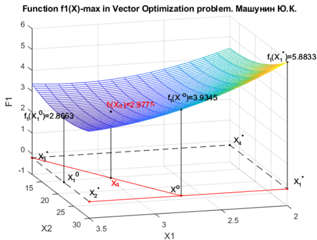
Figure 7. The first characteristics of the f_1(X) technological process in physical units in the three-dimensional coordinate system \{x_1, x_2 \text{ and } f_1(X)\} .
