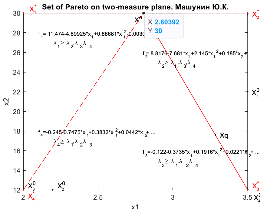
Figure 3. Pareto set, S^0 \subset S in two-dimensional coordinate system, the points of the optimum X_1^* , X_2^* , X_3^* , X_4^* .
