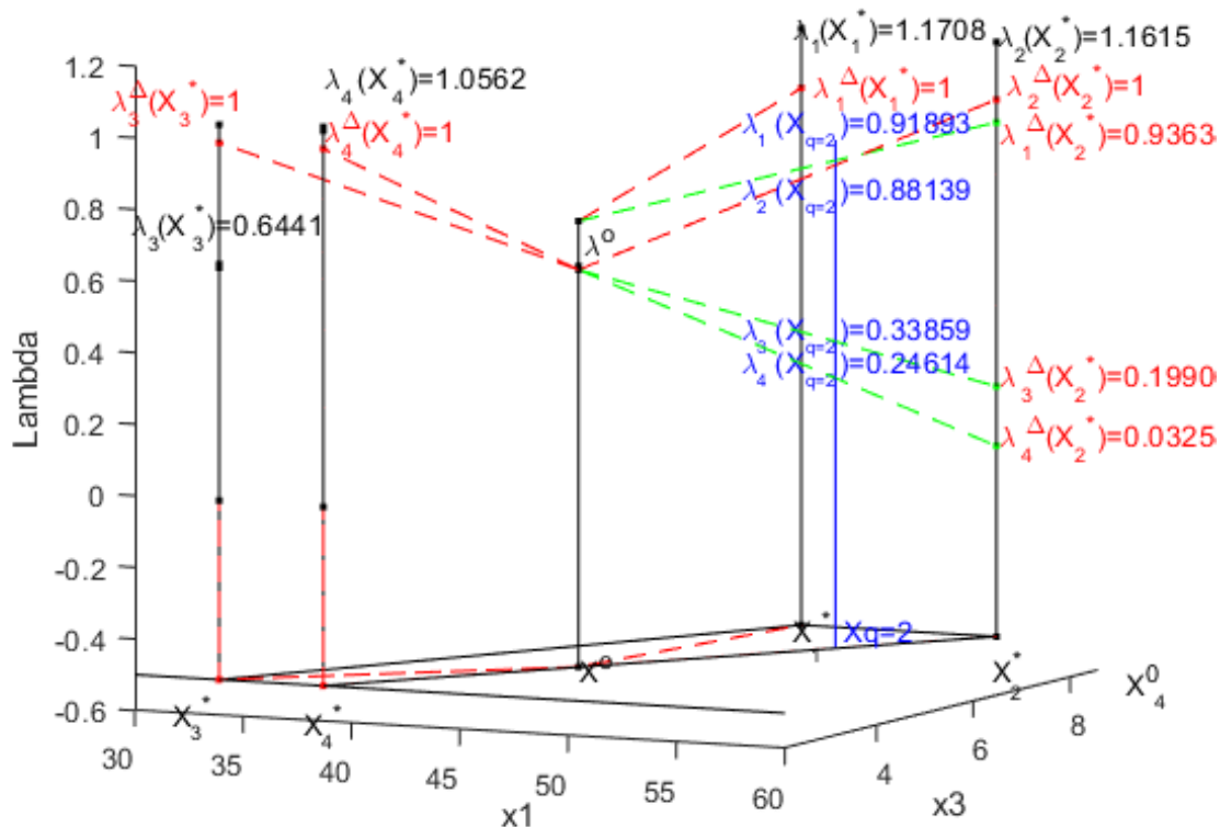
Figure 15.k2. \lambda -problem in the coordinate system x_1 x_3 and \lambda .
