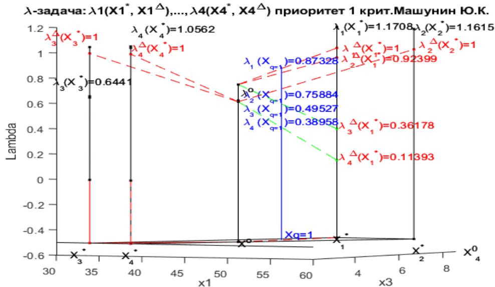
Figure 15.k1. \lambda -problem in the coordinate system x_1 x_3 and \lambda .
