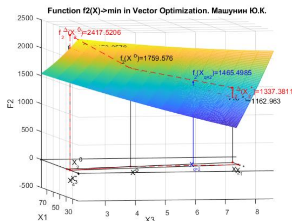
Figure 17.k2. The function f_2(X) with the priority of the second criterion in the two-dimensional coordinate system x_1 x_3 , geometric interpretation of the function f_2(X_{2,q=2}) are coordinates x_1 x_2 x_3 x_4 .
