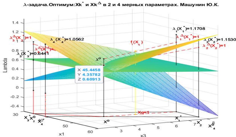
Figure 13. Solving \lambda -problems in a three-dimensional coordinate system x_1, x_3 and \lambda
