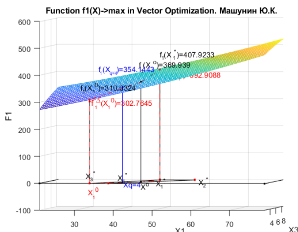
Figure 16.k4. Function f_1(X) with the priority of the fourth criterion in the two-dimensional coordinate system x_1, x_3 and a geometric interpretation of the function f_1(X_{4,q=4}) in the coordinate system x_1, x_2, x_3, x_4 .
