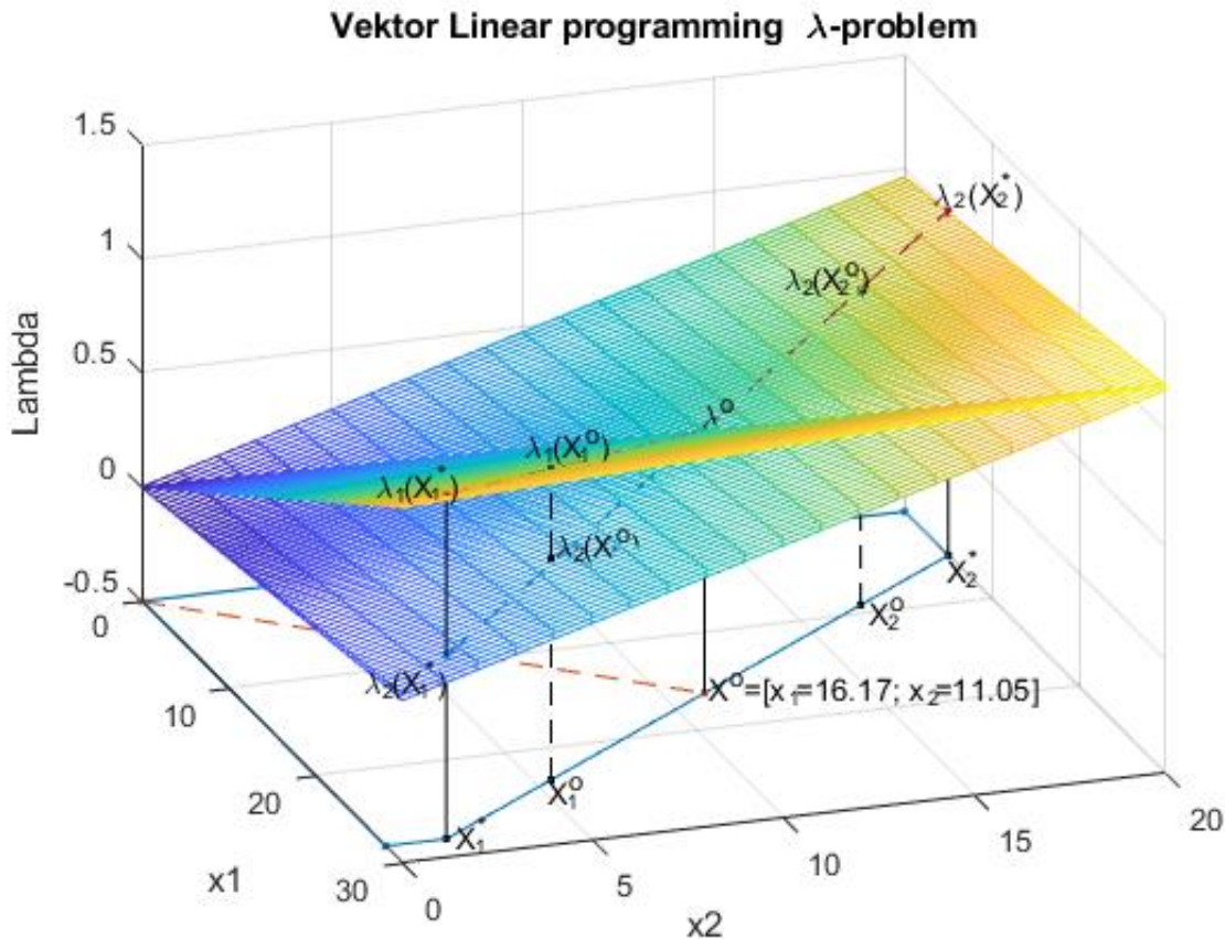
Figure 2. Solution of VPMP (57) and (58) with first-criterion priority
