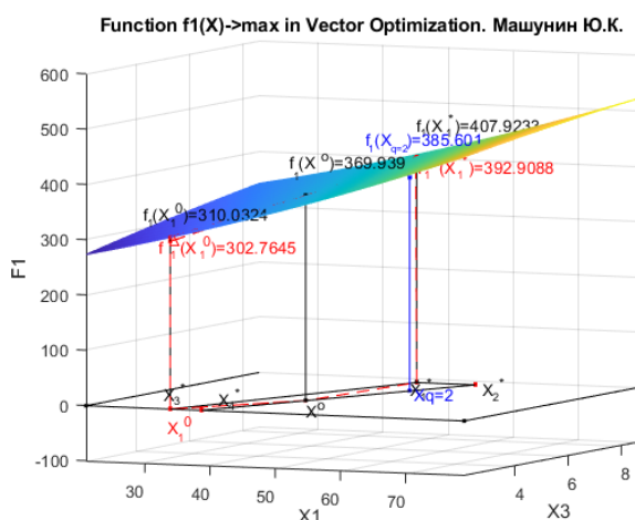
Figure 16.k2. Function f_1(X) with the priority of the second criterion in the two-dimensional coordinate system x_1 x_3 and a geometric interpretation of the function f_1(X_{2,q=2}) in the coordinate system x_1 x_2 x_3 x_4 .
